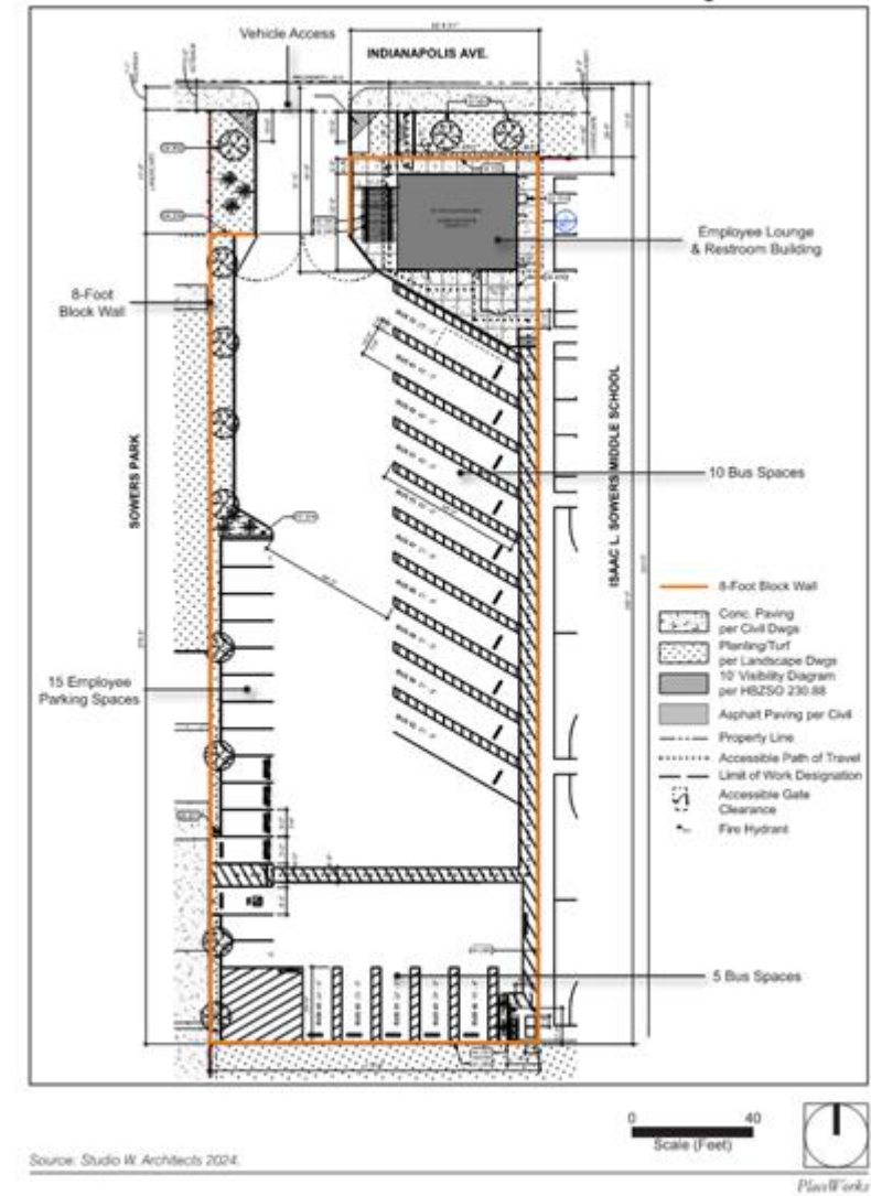
Figure 4 - Site Plan
